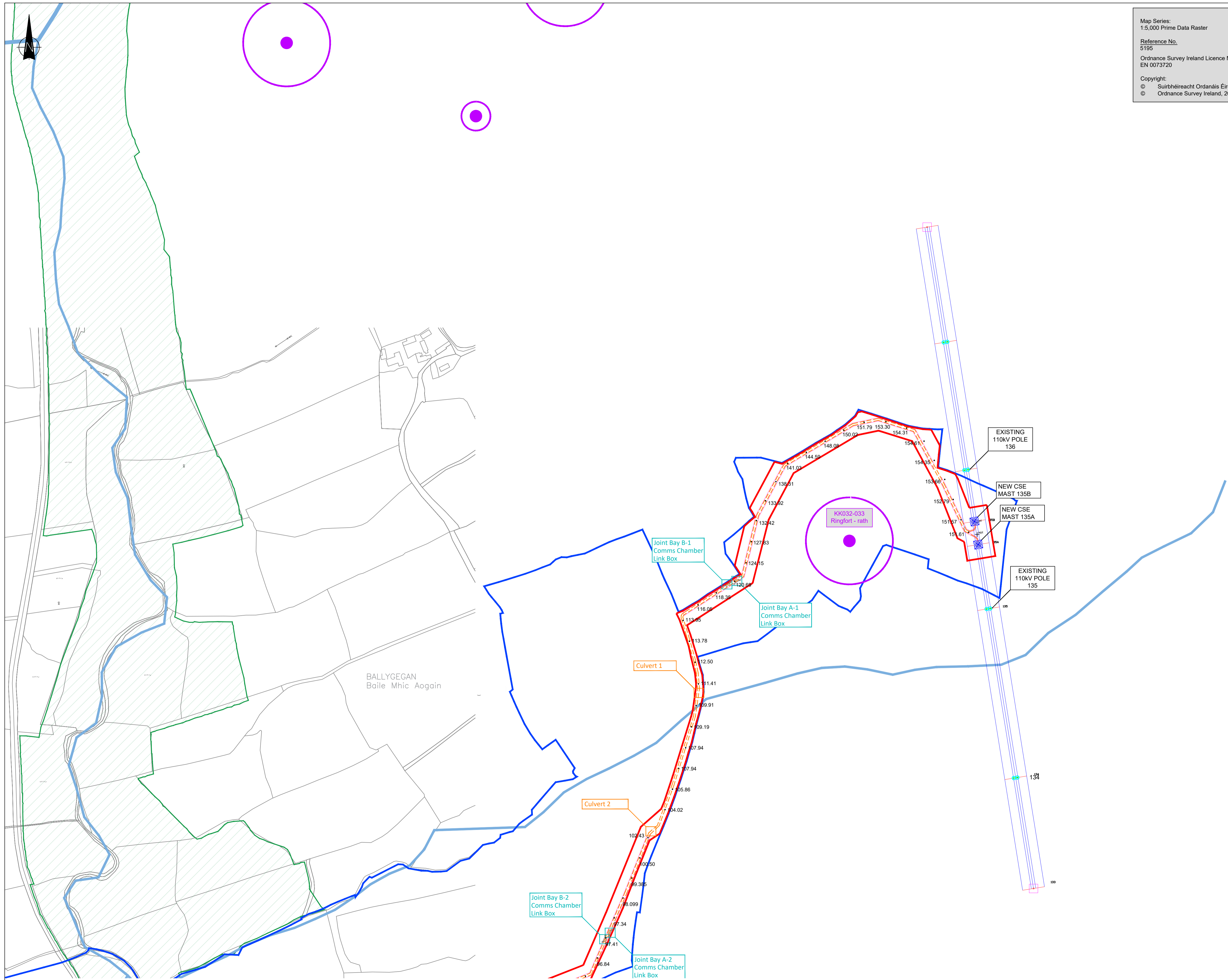
Grid Connection Layout Plan (3 of 3) SCALE :1:2,500
